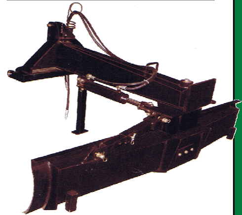
BRB-9 Series Rear Blade Extra Heavy Duty w/ Hydraulic Cylinder
